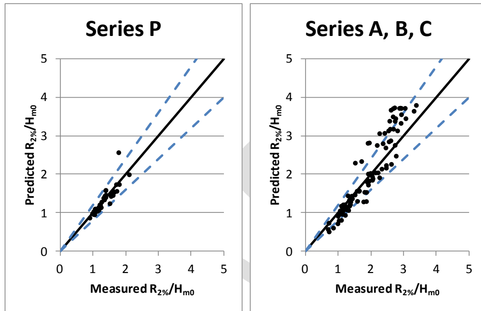
Figure 30. CSHORE predicted relative runup versus van Gent measurements. Solid black line is equality and dashed lines are the 20 percent error.
