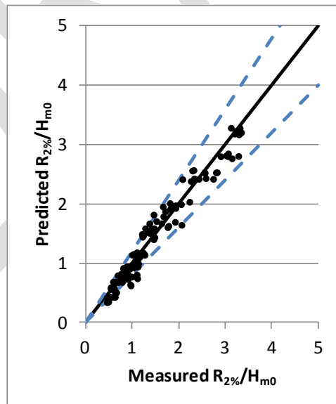
Figure 31. CSHORE predicted relative runup versus Mase measurements. Solid black line is equality and dashed lines are the 20 percent error.
