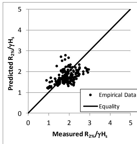
Figure 16. Van der Meer and Stam measured relative runup versus Equations 9 – 11 prediction for H_{m0} at the structure toe and T_p at POS 1 – 3.
