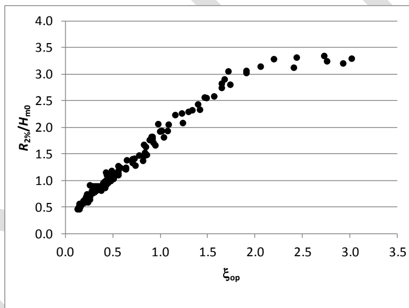
Figure 2. Relative runup versus surf similarity parameter for Mase data set.
