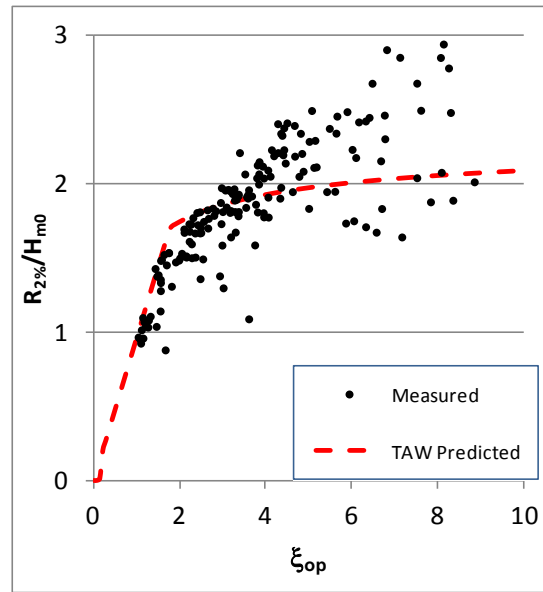
Figure 15. TAW runup prediction plotted with van der Meer and Stam measurements.
