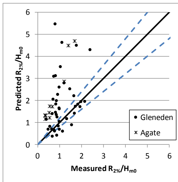
Figure 34. CSHORE predicted runup versus measured during Agate and Gleneden, Oregon, experiments. Solid black line is equality and dashed lines are the 20 percent error.
