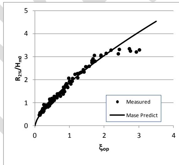
Figure 9. Mase relative runup prediction plotted with Mase measurements.
