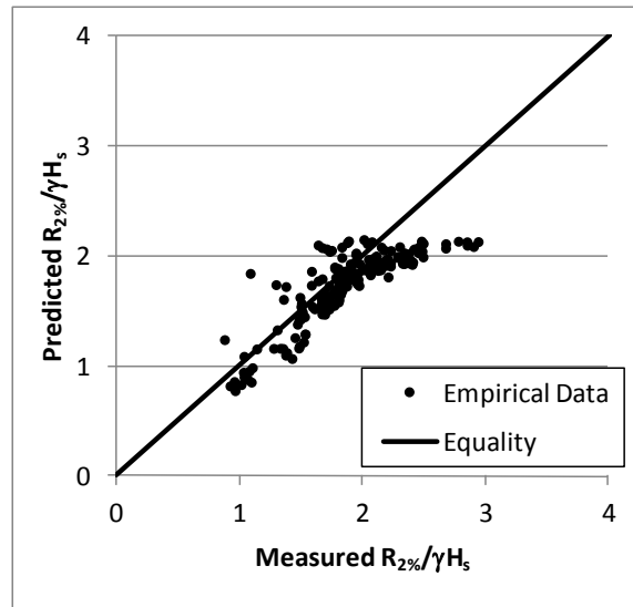
Figure 14. Van der Meer and Stam measured relative runup versus Equation 7 prediction for H_{m0} and T_p at structure toe.
