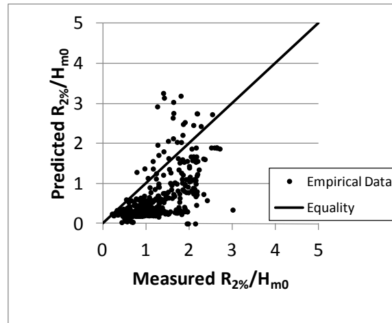
Figure 29. Runup 2.0 prediction versus beach data
