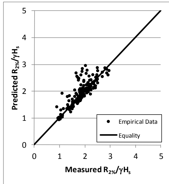
Figure 11. Van der Meer and Stam measured relative runup versus Equation 6.
