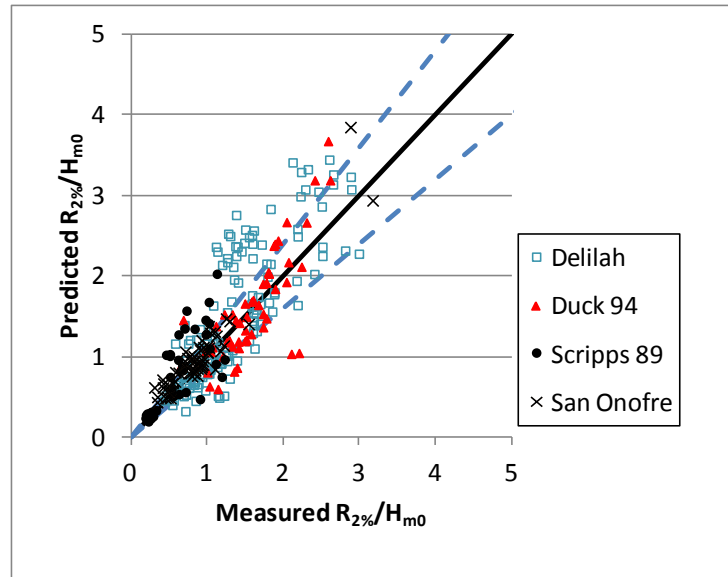
Figure 32. CSHORE predicted runup versus measured runup during Duck 1990, Duck 1994, Scripps, and San Onofre experiments. Solid black line is equality and dashed lines are the 20 percent error.
