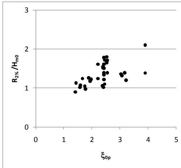
Figure 4. Relative runup versus surf similarity parameter for van Gent Series P.
