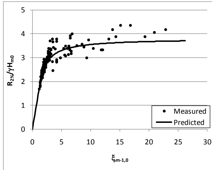
Figure 12. Equation 7 relative runup prediction plotted with van Gent measurements.
