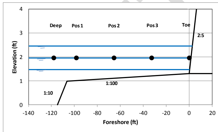
Figure 18. Van Gent Series B nearshore layout with wave gage location.
