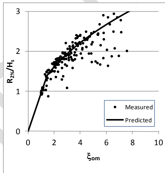
Figure 10. Van der Meer and Stam relative runup prediction using Equation 6 plotted with their measurements.
