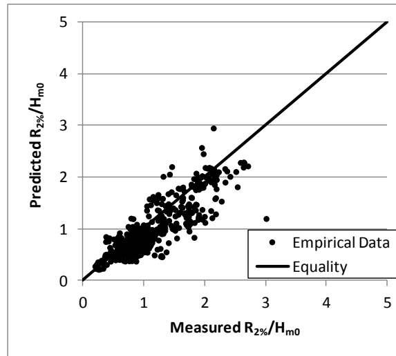
Figure 25. Fit of Stockdon equations to Stockdon beach data.
