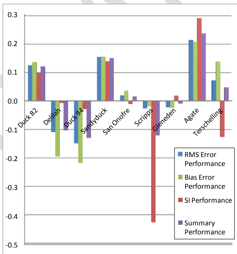
Figure 26. Skill comparison for modified Mase Equation 4 (with a = 1.1 , b = 0.7 and c = 0 ) vs Stockdon Equation 30. The value plotted is 1 - X_M/X_S where X_M is the skill score for Equation 4 and X_S is the skill score for Equation 30.
