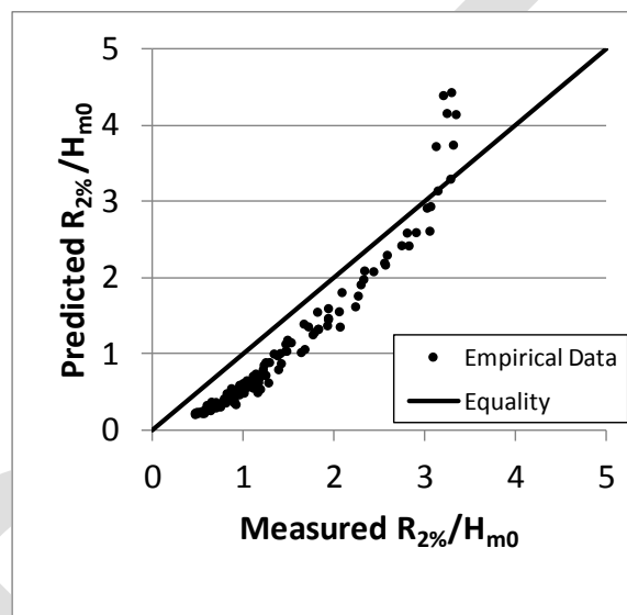
Figure 27. Runup 2.0 prediction versus Mase smooth uniform slope data.
