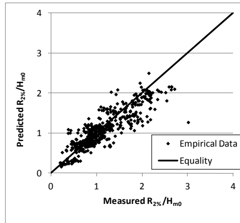
Figure 21. Fit 4 relative runup prediction plotted against Stockdon measurements.
