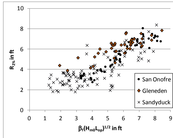
Figure 23. Dimensional runup as a function of \beta_1(H_{m0}L_{op})^{1/2} for incident-wave-dominated experiments at disparate sites.
