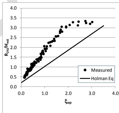
Figure 19. Holman relative runup prediction plotted with Mase measurements.
