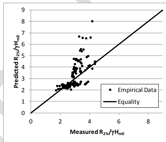
Figure 17. Van Gent measured relative runup versus Equations 9 – 11 prediction for H_{m0} at the structure toe and T_p at POS 1 – 3.
