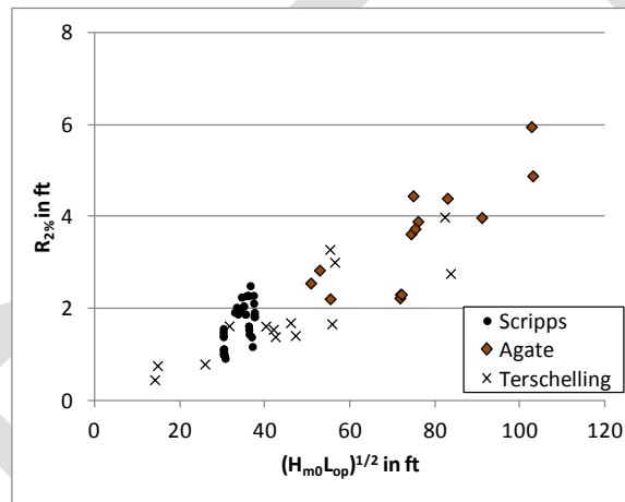
Figure 24. Dimensional runup as a function of (H_{m0}L_{op})^{1/2} for infragravity-wave-dominated experiments.
