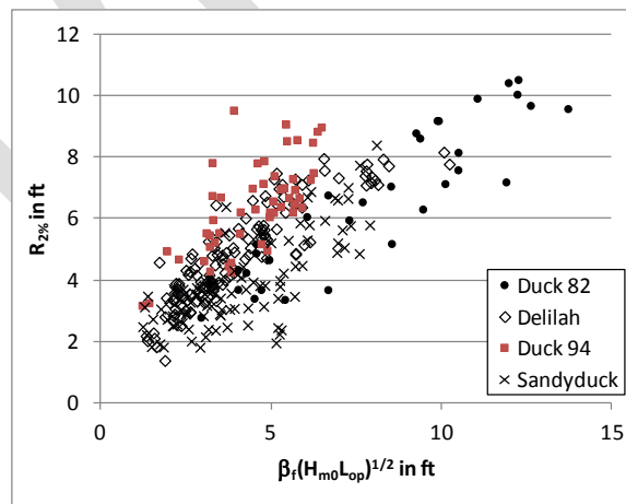
Figure 22. Dimensional runup as a function of \beta_f(H_{m0}L_{op})^{1/2} for incident-wave-dominated experiments at Duck, NC.
