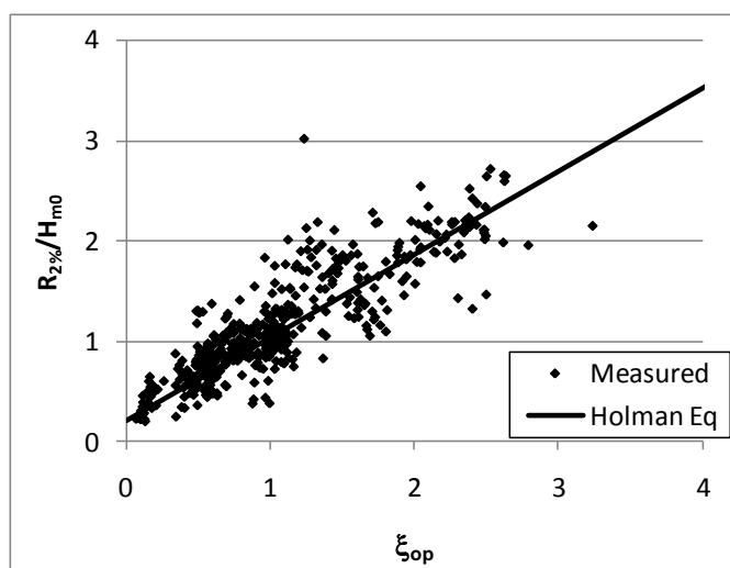
Figure 20. Holman relative runoff prediction plotted with Stockdon measurements.
