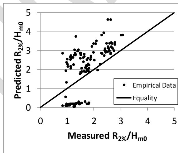
Figure 28. Runup 2.0 prediction versus van Gent smooth structure data.
