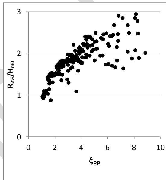
Figure 3. Relative runup versus surf similarity parameter for van der Meer and Stam for rubble mound structure experiments.
