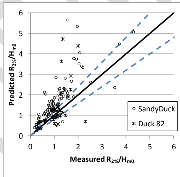
Figure 33. CSHORE predicted runup versus measured during Duck 1982 and SandyDuck experiments. Solid black line is equality and dashed lines are the 20 percent error.
