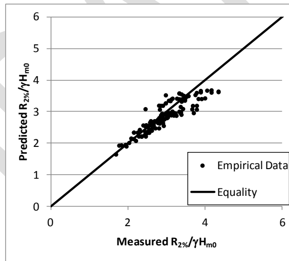
Figure 13. Van Gent measured relative runup versus Equation 7 prediction for H_{m0} and T_{m-1,0} at structure toe.
